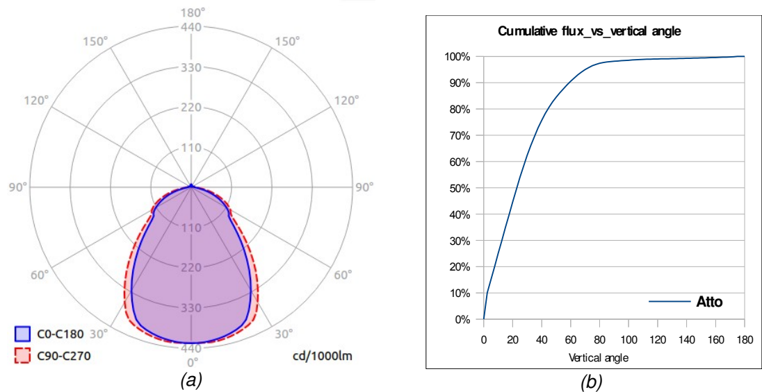
Fig. 5. (a) Light distribution curve of Atto 5000. Light distribution is shown in two perpendicular vertical planes (C-planes). (b) Cumulative light flux (%) vs. vertical angle.
